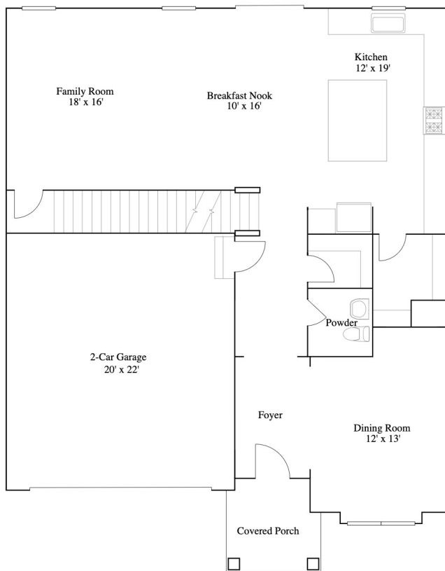
1st Floor
